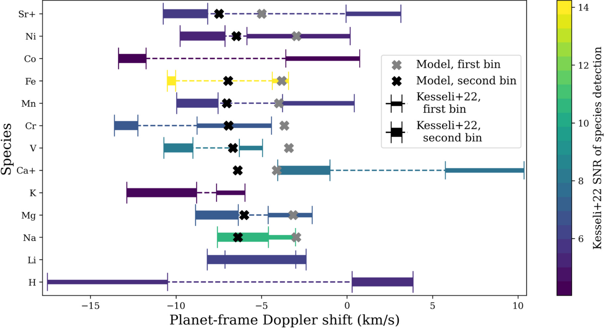
Figure 8. from Arjun B. Savel et al 2023 Astrophys. J. 944 doi:10.3847/1538-4357/acb141 https://dx.doi.org/10.3847/1538-4357/acb141 © 2023. The Author(s). Published by the American Astronomical Society.
