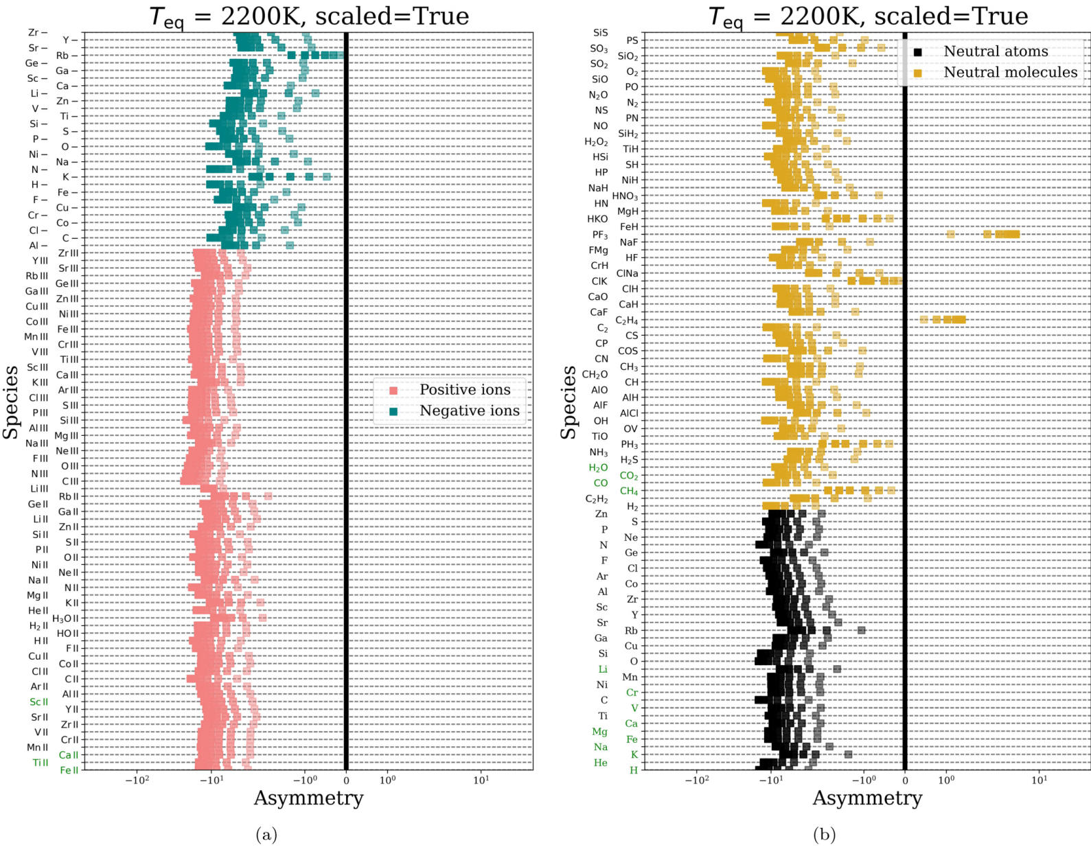
Figure 2. from Arjun B. Savel et al 2023 Astrophys. J. 944 doi:10.3847/1538-4357/acb141 https://dx.doi.org/10.3847/1538-4357/acb141 © 2023. The Author(s). Published by the American Astronomical Society.
