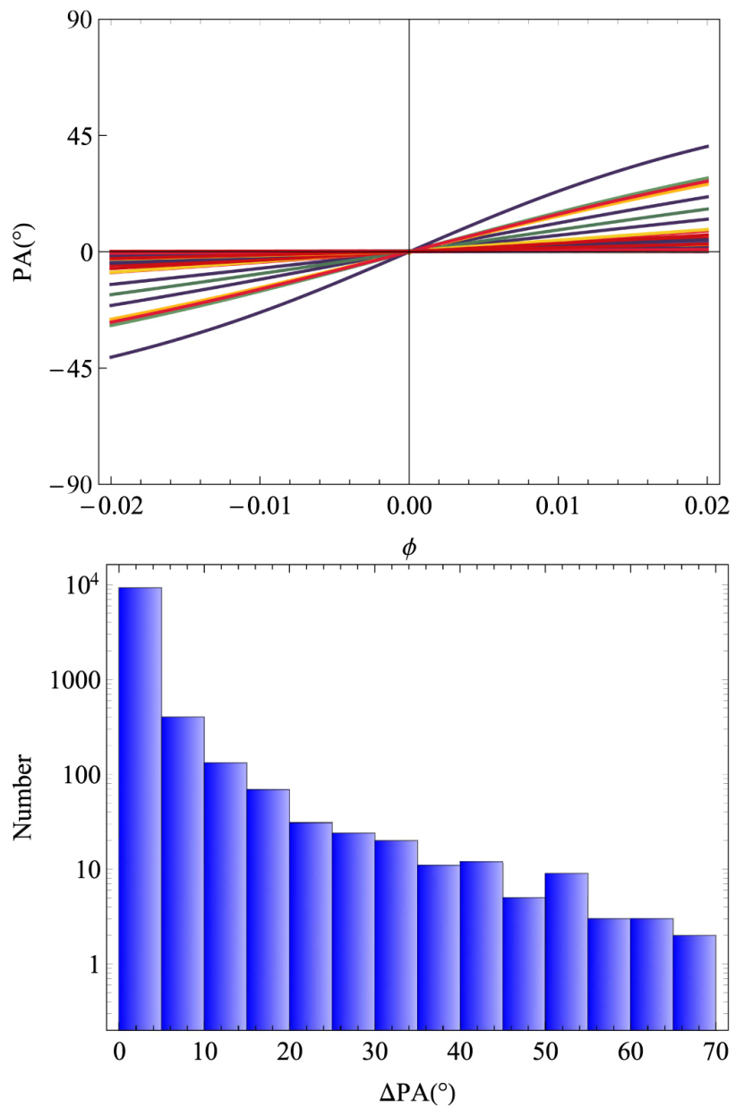
Figure 8. from Ze-Nan Liu et al 2023 Astrophys. J. 943 doi:10.3847/1538-4357/acac23 https://dx.doi.org/10.3847/1538-4357/acac23 © 2023. The Author(s). Published by the American Astronomical Society.
