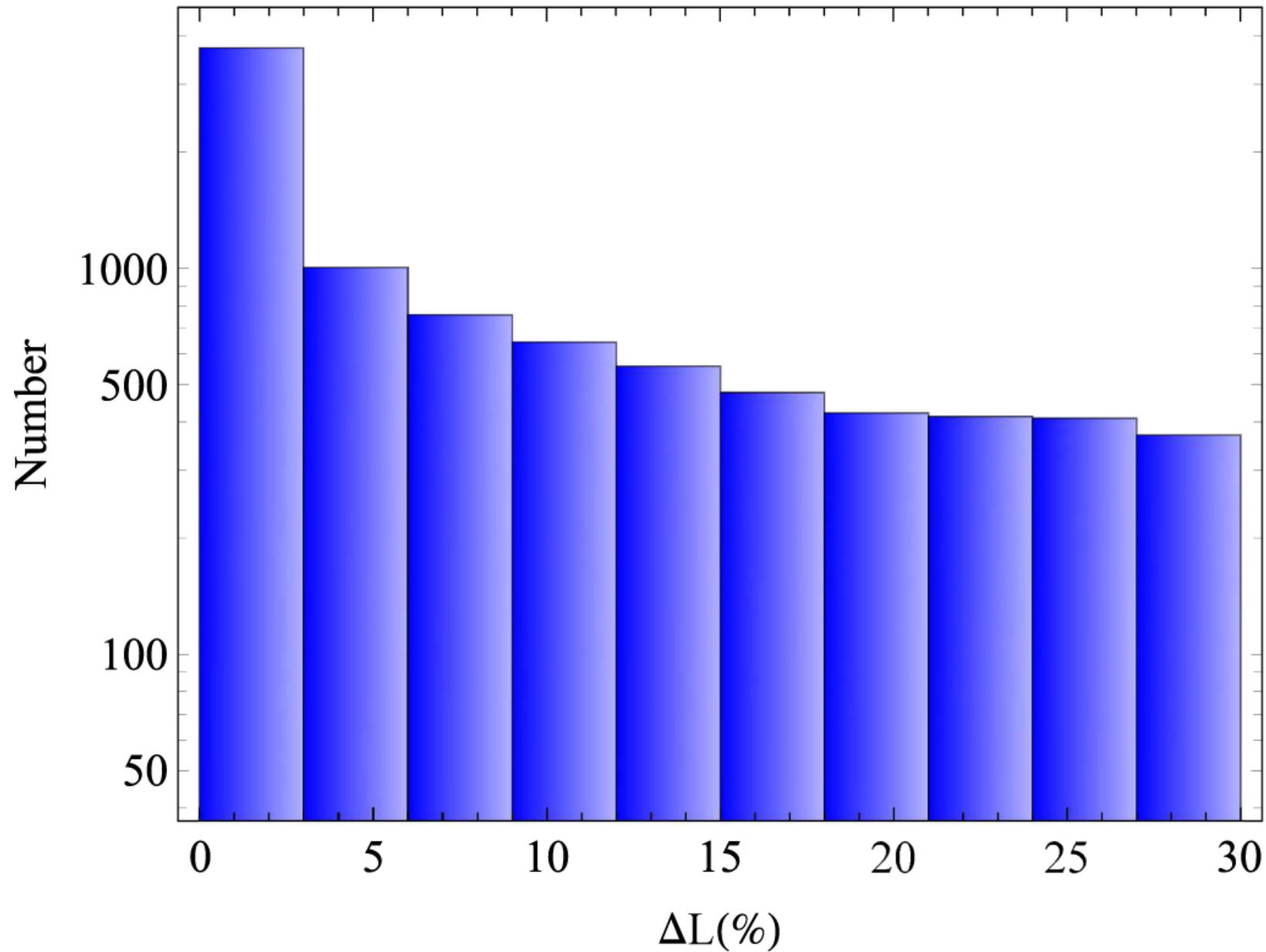
Figure 7. from Ze-Nan Liu et al 2023 Astrophys. J. 943 doi:10.3847/1538-4357/acac23 https://dx.doi.org/10.3847/1538-4357/acac23 © 2023. The Author(s). Published by the American Astronomical Society.
