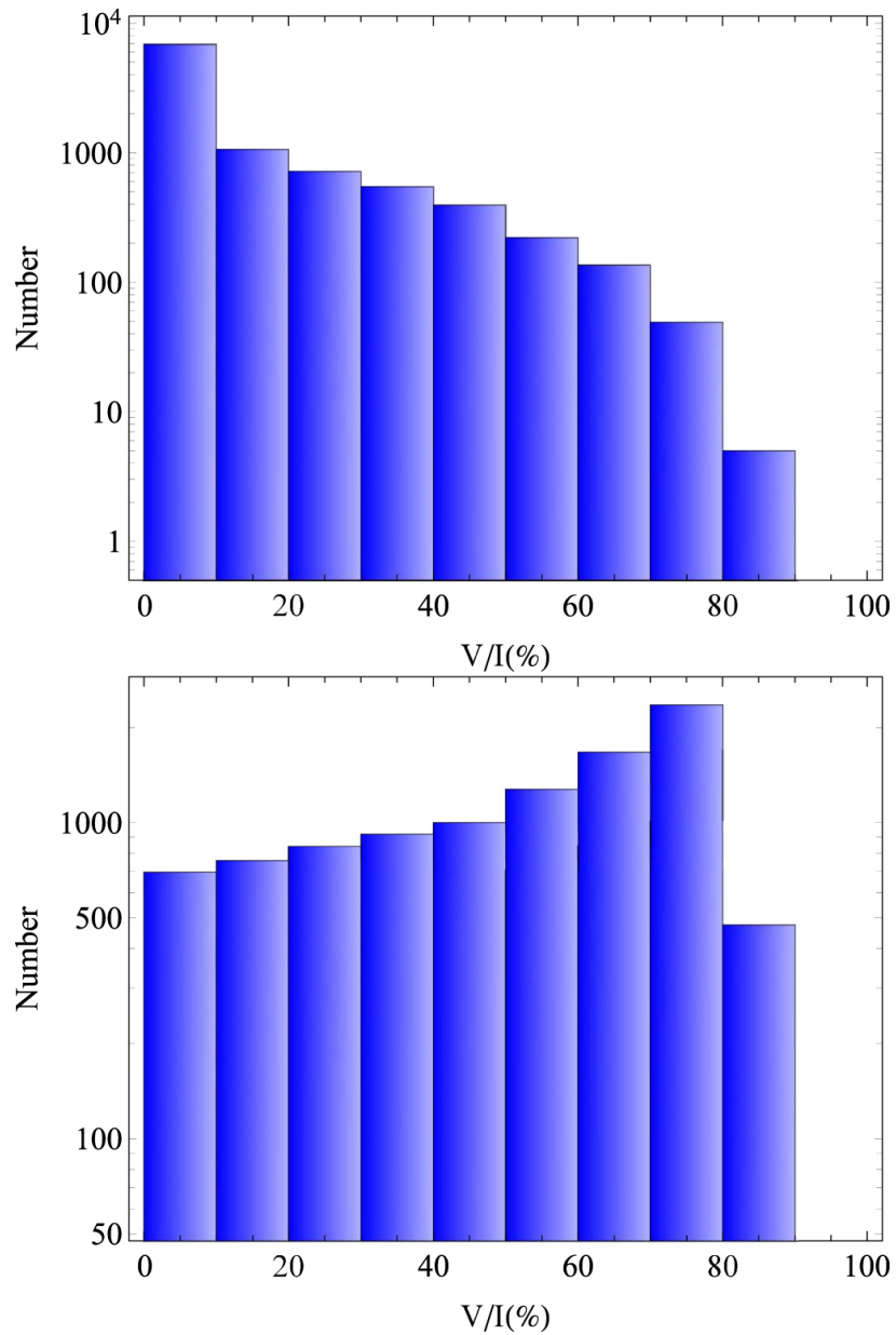
Figure 5. from Ze-Nan Liu et al 2023 Astrophys. J. 943 doi:10.3847/1538-4357/acac23 https://dx.doi.org/10.3847/1538-4357/acac23 © 2023. The Author(s). Published by the American Astronomical Society.
