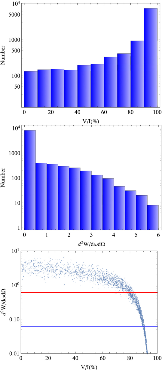
Figure 4. from Ze-Nan Liu et al 2023 Astrophys. J. 943 doi:10.3847/1538-4357/acac23 https://dx.doi.org/10.3847/1538-4357/acac23 © 2023. The Author(s). Published by the American Astronomical Society.
