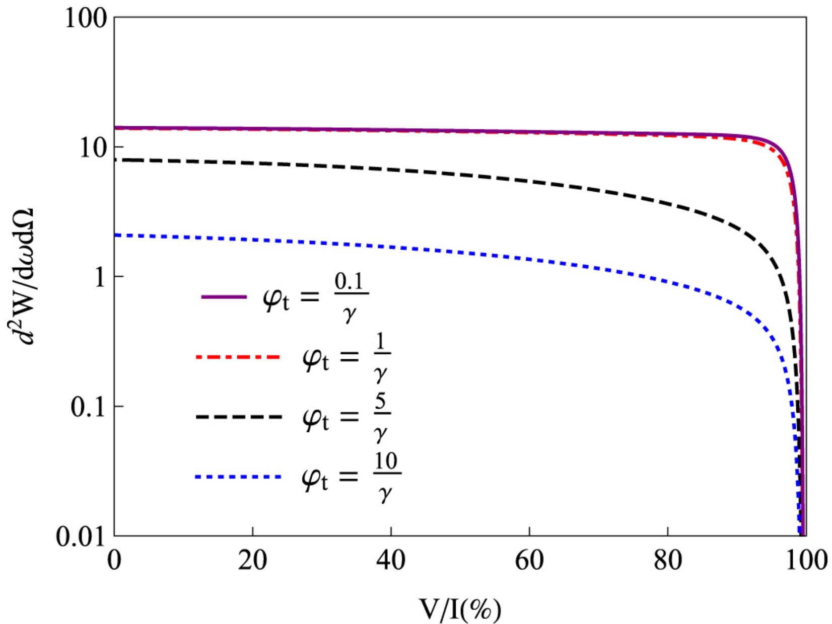
Figure 3. from Ze-Nan Liu et al 2023 Astrophys. J. 943 doi:10.3847/1538-4357/acac23 https://dx.doi.org/10.3847/1538-4357/acac23 © 2023. The Author(s). Published by the American Astronomical Society.
