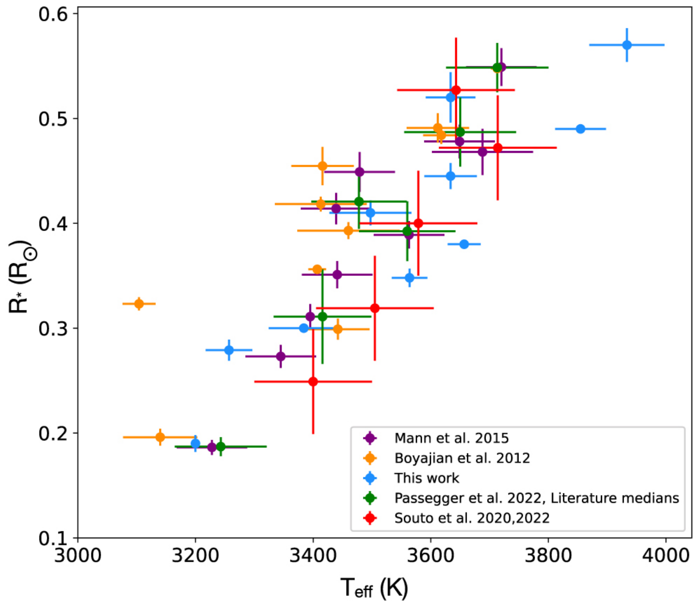
Figure 9. from Aishwarya R. Iyer et al 2023 Astrophys. J. 944 doi:10.3847/1538-4357/acabc2 https://dx.doi.org/10.3847/1538-4357/acabc2 © 2023. The Author(s). Published by the American Astronomical Society.
