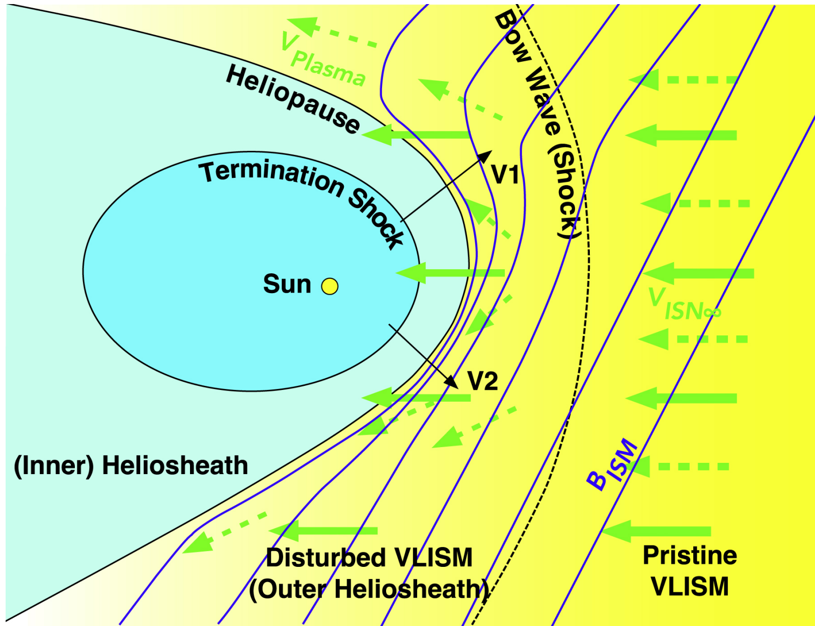
Figure 1. from Jeffrey L. Linsky and Eberhard Moebius 2023 Astrophys. J. 942 doi:10.3847/1538-4357/aca676 https://dx.doi.org/10.3847/1538-4357/aca676 © 2023. The Author(s). Published by the American Astronomical Society.
