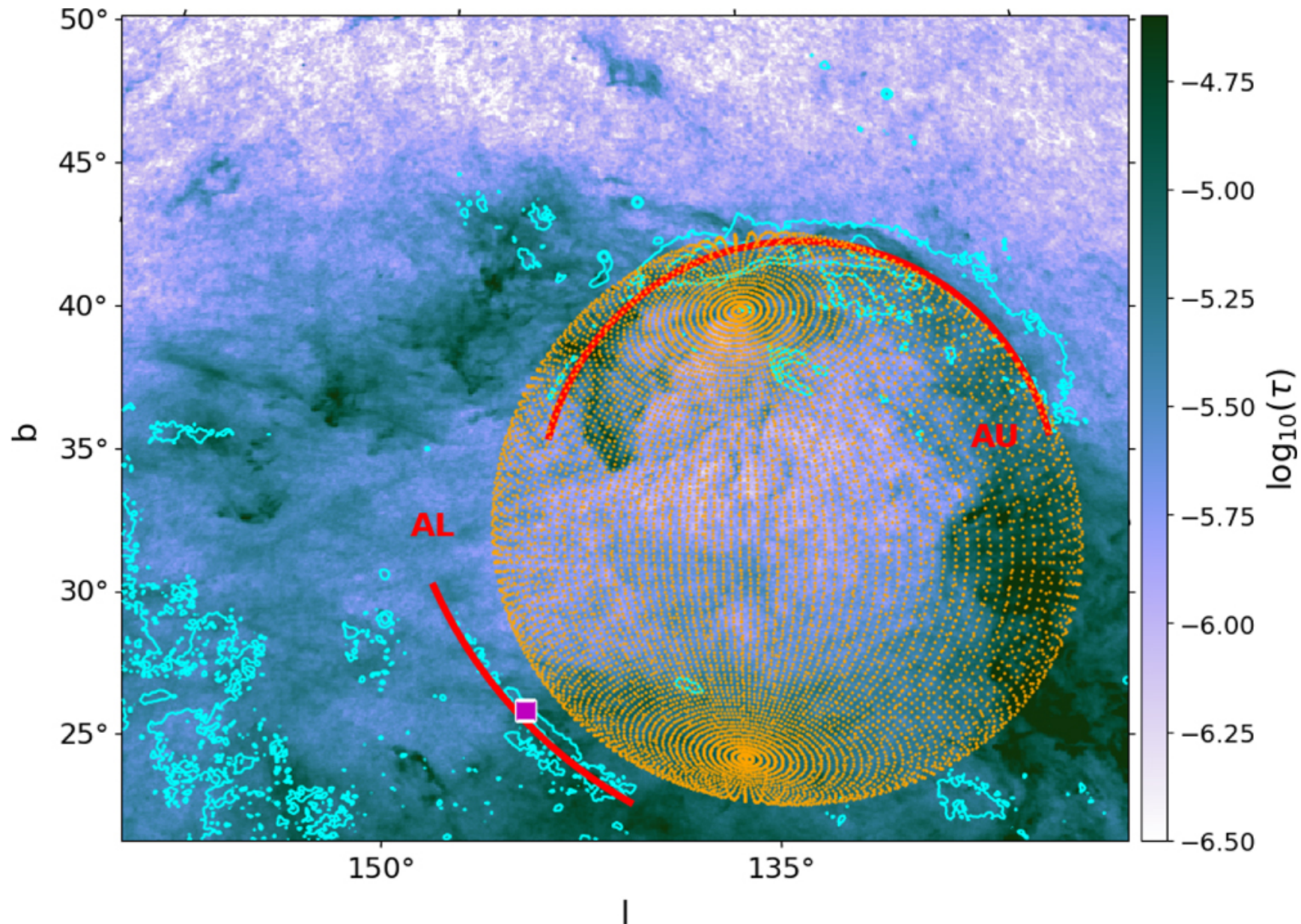
Figure 8. from Antoine Marchal and Peter G. Martin 2023 Astrophys. J. 942 doi:10.3847/1538-4357/aca4d2 https://dx.doi.org/10.3847/1538-4357/aca4d2 © 2023. The Author(s). Published by the American Astronomical Society.
