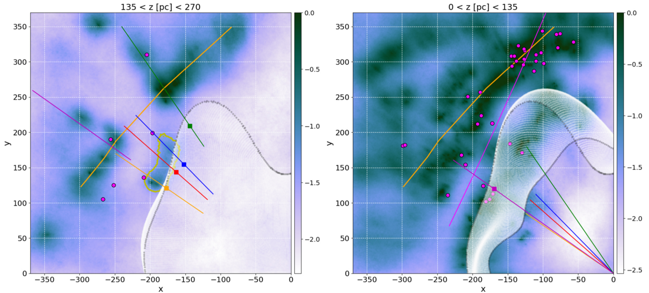
Figure 6. from Antoine Marchal and Peter G. Martin 2023 Astrophys. J. 942 doi:10.3847/1538-4357/aca4d2 https://dx.doi.org/10.3847/1538-4357/aca4d2 © 2023. The Author(s). Published by the American Astronomical Society.
