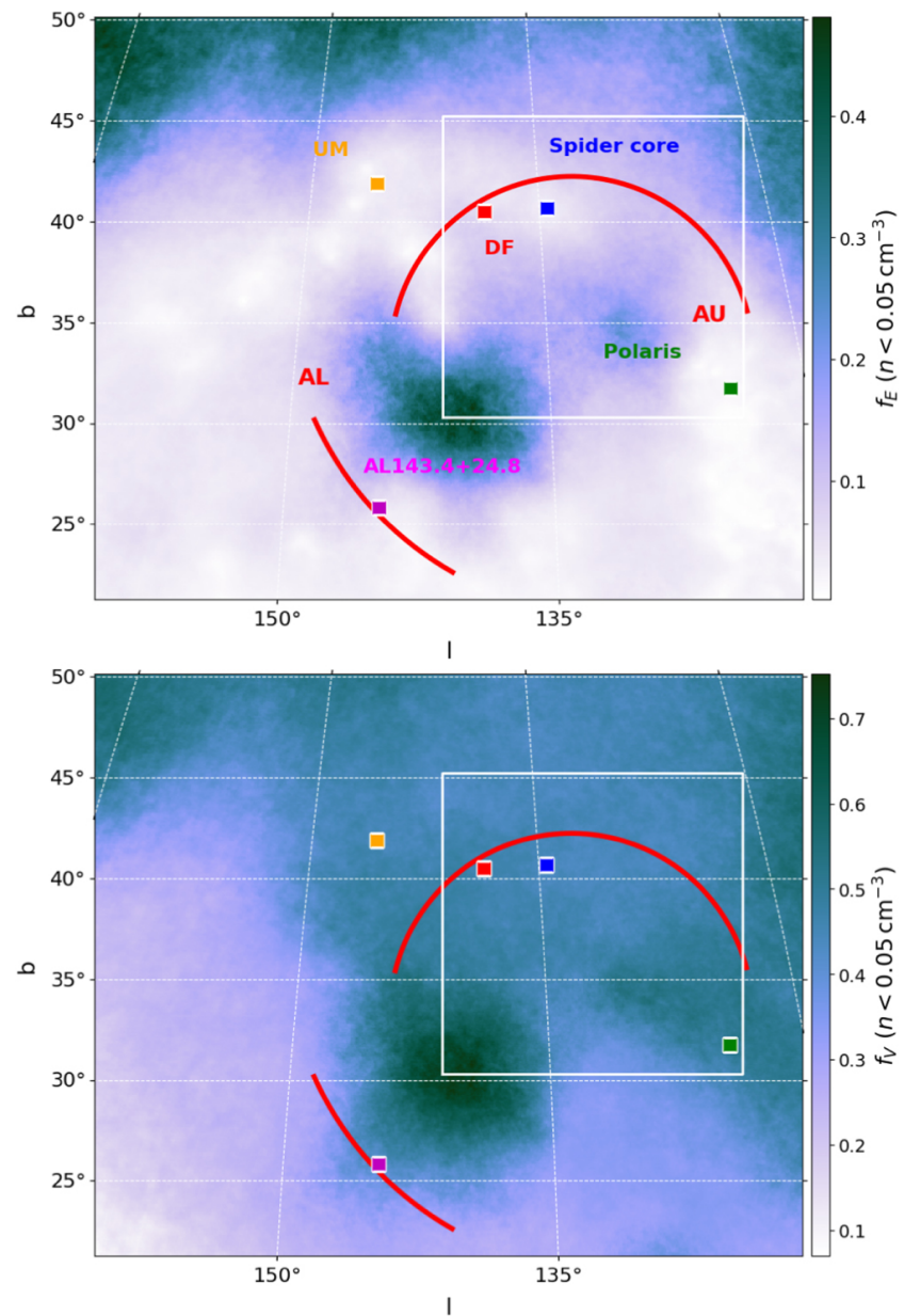
Figure 5. from Antoine Marchal and Peter G. Martin 2023 Astrophys. J. 942 doi:10.3847/1538-4357/aca4d2 https://dx.doi.org/10.3847/1538-4357/aca4d2 © 2023. The Author(s). Published by the American Astronomical Society.
