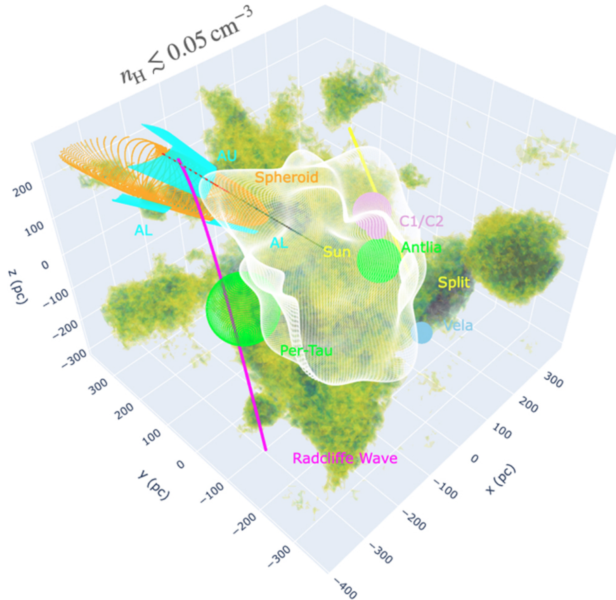
Figure 13. from Antoine Marchal and Peter G. Martin 2023 Astrophys. J. 942 doi:10.3847/1538-4357/aca4d2 https://dx.doi.org/10.3847/1538-4357/aca4d2 © 2023. The Author(s). Published by the American Astronomical Society.
