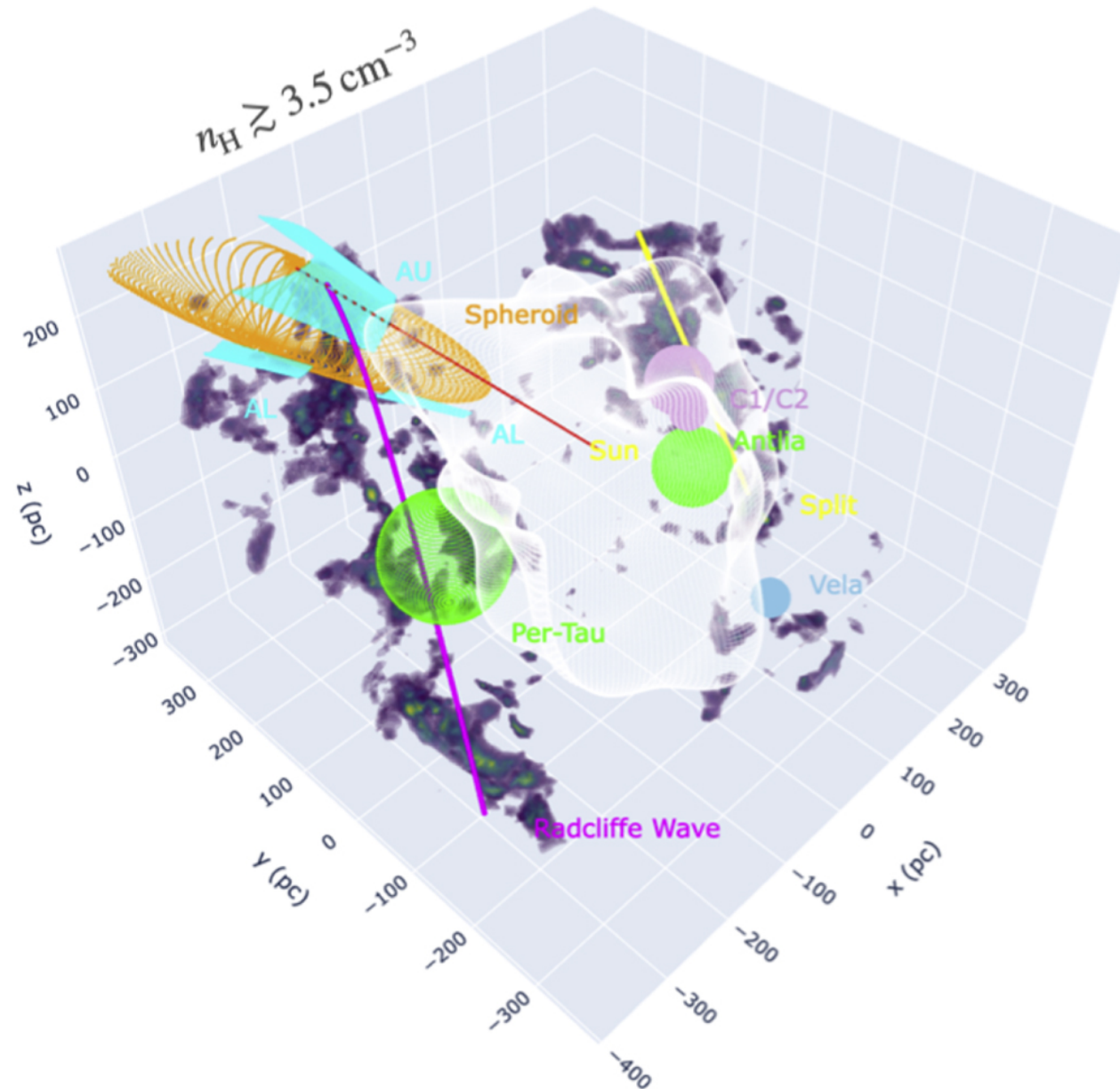
Figure 12. from Antoine Marchal and Peter G. Martin 2023 Astrophys. J. 942 doi:10.3847/1538-4357/aca4d2 https://dx.doi.org/10.3847/1538-4357/aca4d2 © 2023. The Author(s). Published by the American Astronomical Society.
