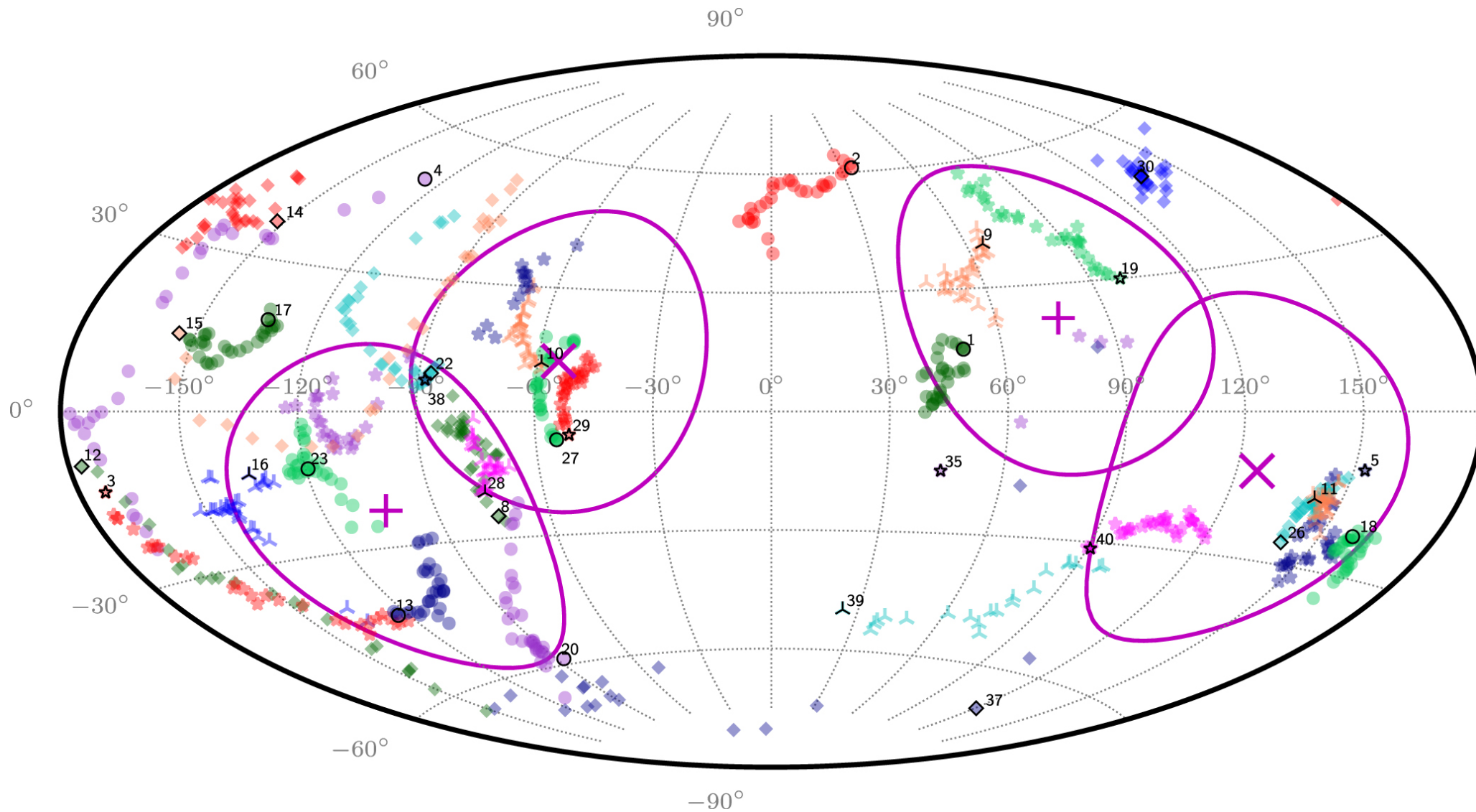
Figure A1. from Isabel Santos-Santos et al 2023 Astrophys. J. 942 doi:10.3847/1538-4357/aca1c8 https://dx.doi.org/10.3847/1538-4357/aca1c8 © 2023. The Author(s). Published by the American Astronomical Society.
