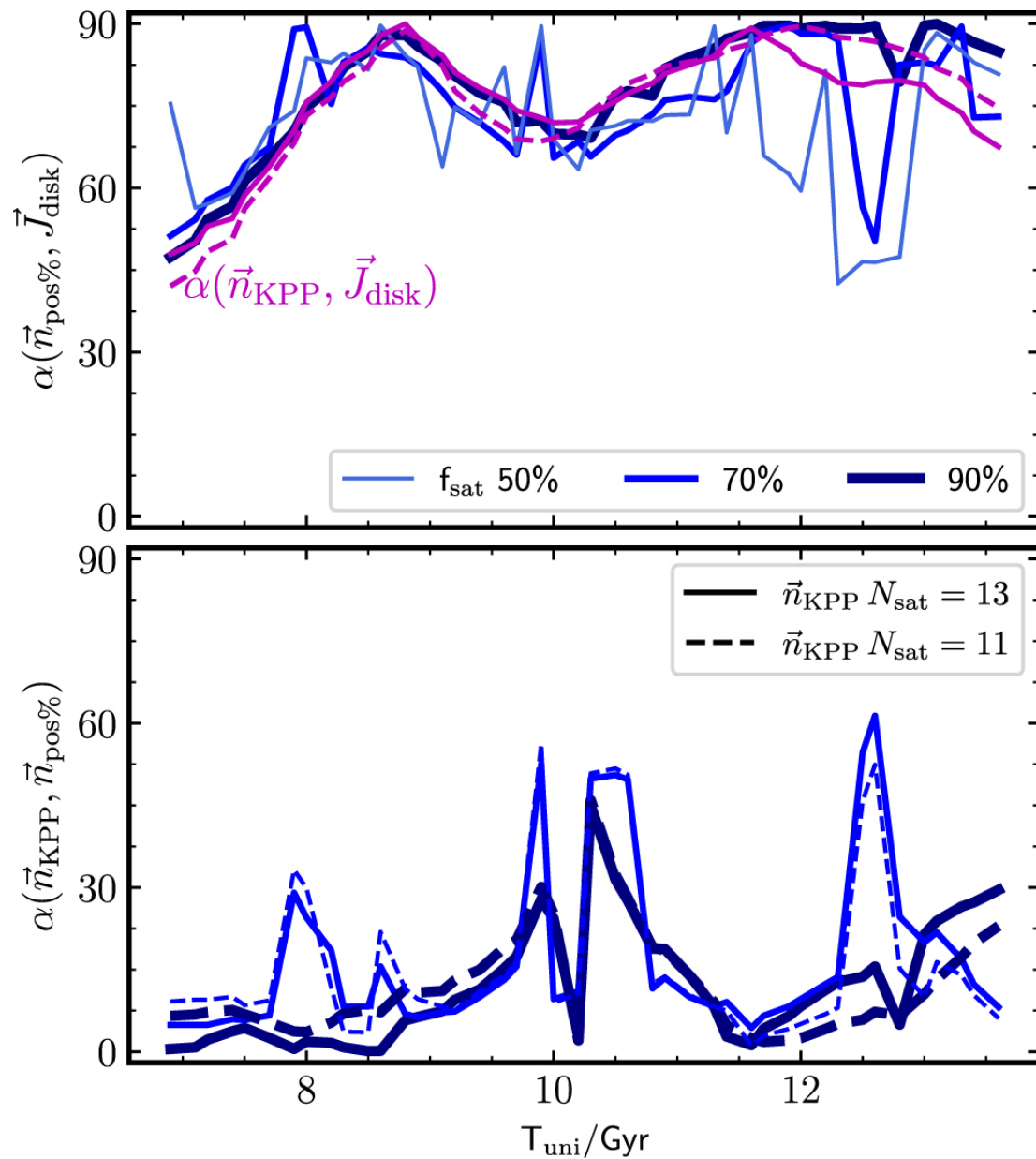
Figure 7. from Isabel Santos-Santos et al 2023 Astrophys. J. 942 doi:10.3847/1538-4357/aca1c8 https://dx.doi.org/10.3847/1538-4357/aca1c8 © 2023. The Author(s). Published by the American Astronomical Society.
