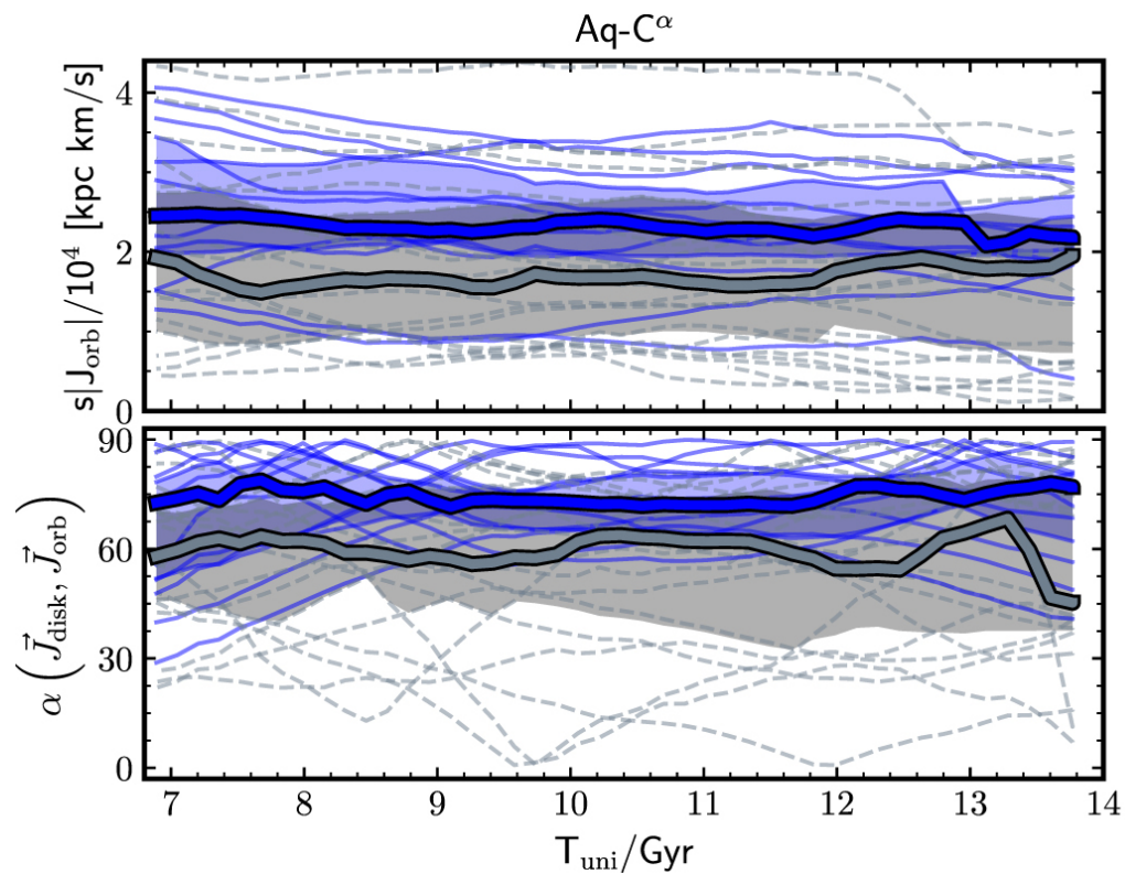
Figure 5. from Isabel Santos-Santos et al 2023 Astrophys. J. 942 doi:10.3847/1538-4357/aca1c8 https://dx.doi.org/10.3847/1538-4357/aca1c8 © 2023. The Author(s). Published by the American Astronomical Society.
