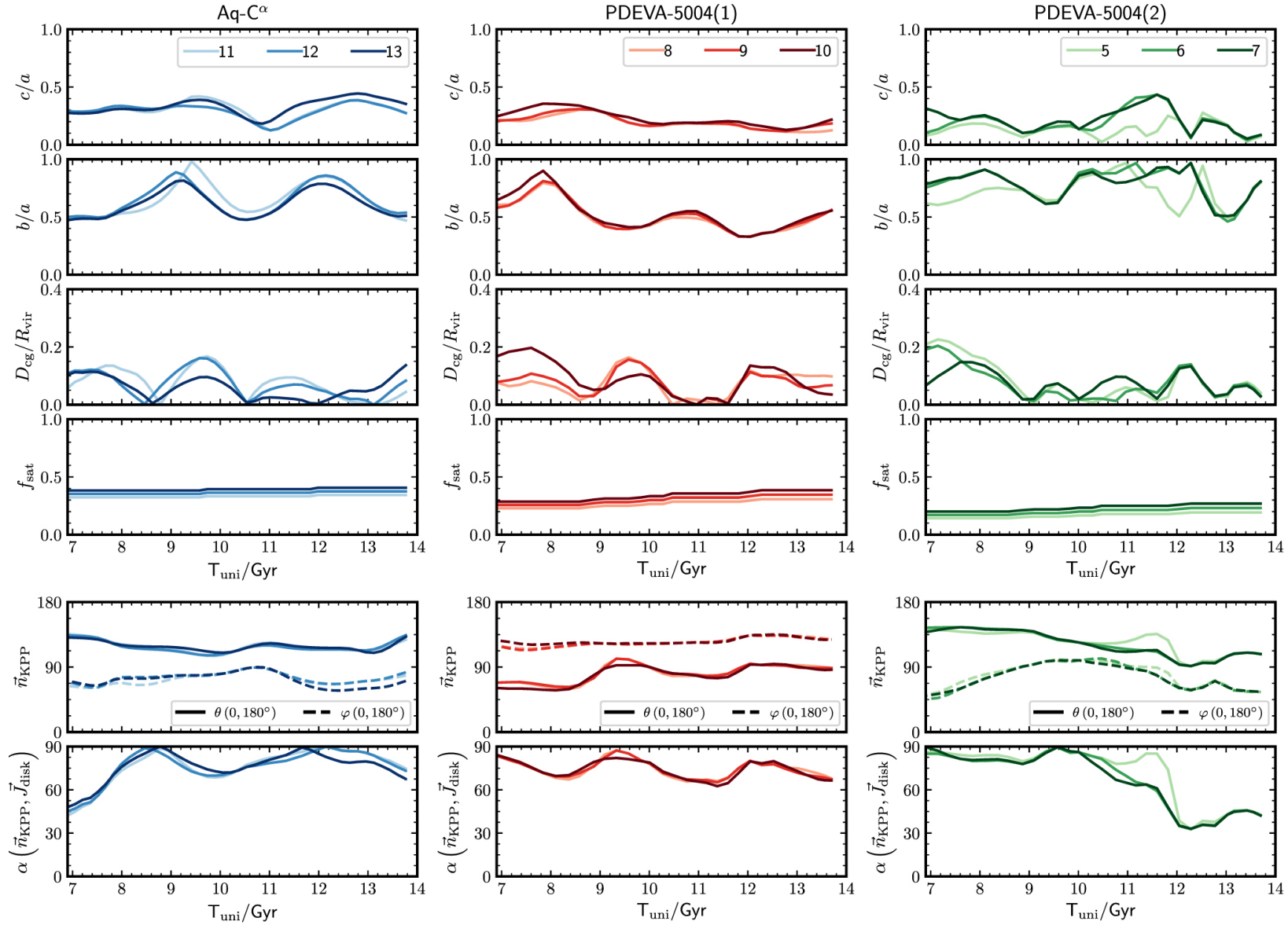
Figure 4. from Isabel Santos-Santos et al 2023 Astrophys. J. 942 doi:10.3847/1538-4357/aca1c8 https://dx.doi.org/10.3847/1538-4357/aca1c8 © 2023. The Author(s). Published by the American Astronomical Society.
