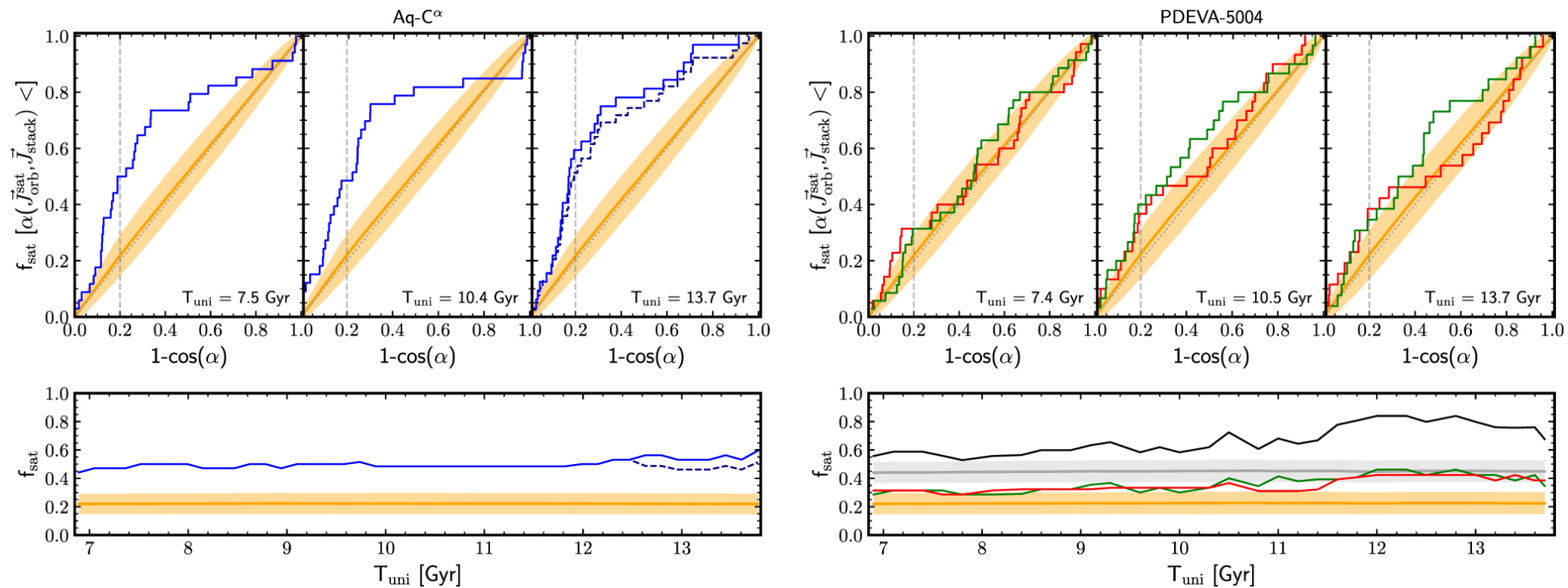
Figure 3. from Isabel Santos-Santos et al 2023 Astrophys. J. 942 doi:10.3847/1538-4357/aca1c8 https://dx.doi.org/10.3847/1538-4357/aca1c8 © 2023. The Author(s). Published by the American Astronomical Society.
