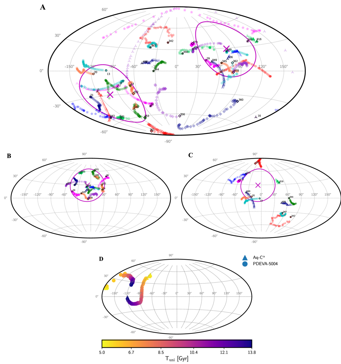
Figure 2. from Isabel Santos-Santos et al 2023 Astrophys. J. 942 doi:10.3847/1538-4357/aca1c8 https://dx.doi.org/10.3847/1538-4357/aca1c8 © 2023. The Author(s). Published by the American Astronomical Society.
