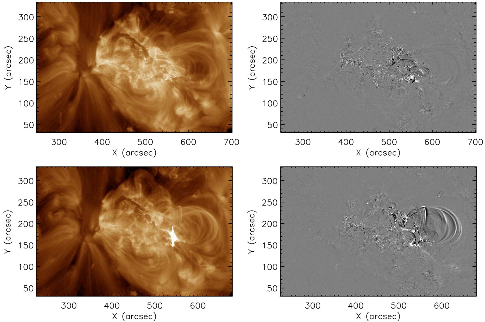
Figure 8. from Karin Dissauer et al 2023 Astrophys. J. 942 doi:10.3847/1538-4357/ac9c06 https://dx.doi.org/10.3847/1538-4357/ac9c06 © 2023. The Author(s). Published by the American Astronomical Society.
