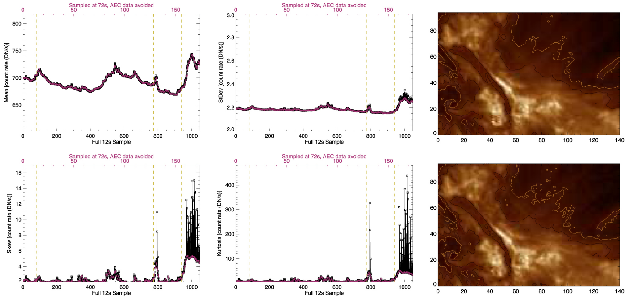
Figure 4. from Karin Dissauer et al 2023 Astrophys. J. 942 doi:10.3847/1538-4357/ac9c06 https://dx.doi.org/10.3847/1538-4357/ac9c06 © 2023. The Author(s). Published by the American Astronomical Society.
