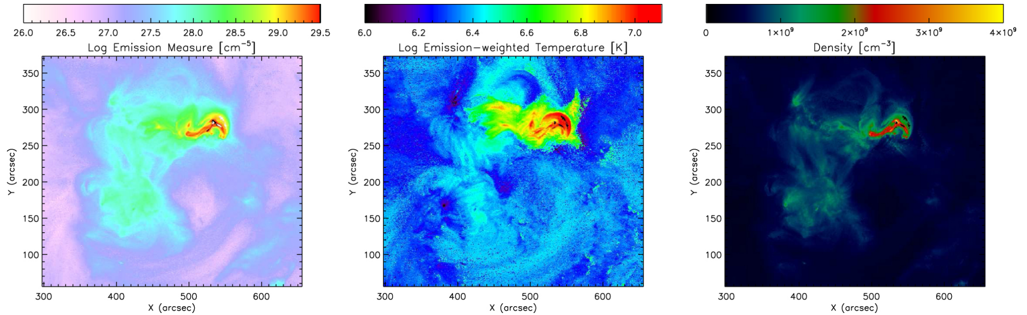
Figure 3. from Karin Dissauer et al 2023 Astrophys. J. 942 doi:10.3847/1538-4357/ac9c06 https://dx.doi.org/10.3847/1538-4357/ac9c06 © 2023. The Author(s). Published by the American Astronomical Society.
