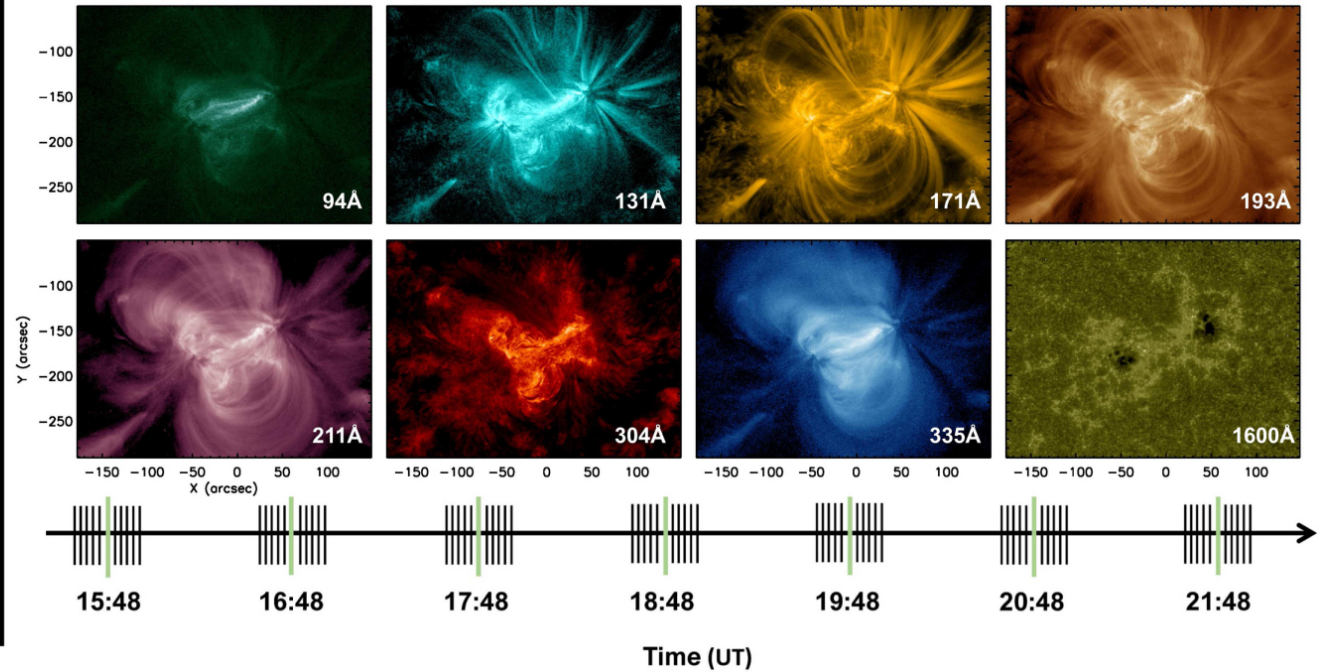
Figure 1. from Karin Dissauer et al 2023 Astrophys. J. 942 doi:10.3847/1538-4357/ac9c06 https://dx.doi.org/10.3847/1538-4357/ac9c06 © 2023. The Author(s). Published by the American Astronomical Society.
