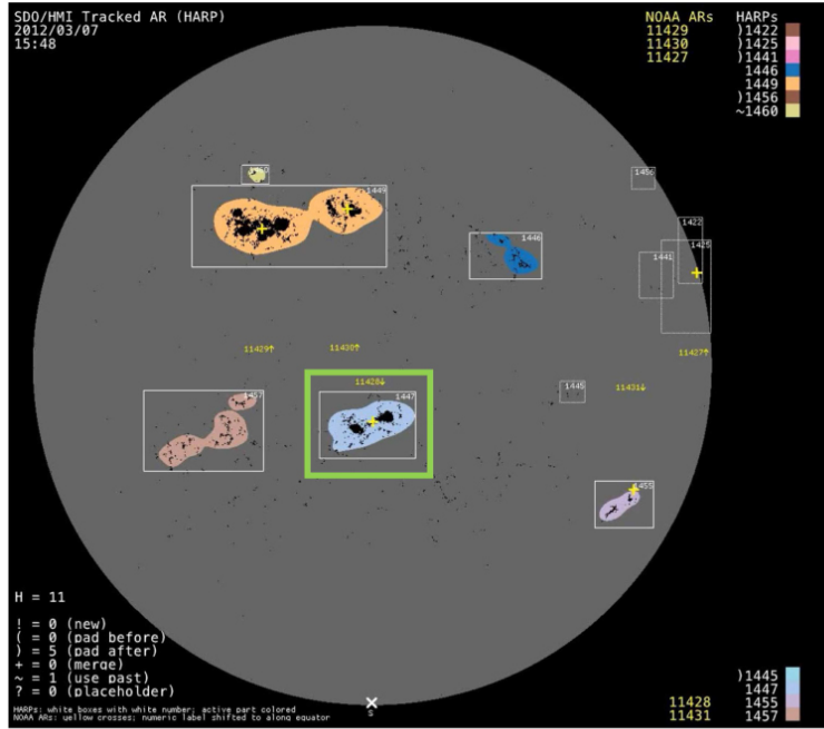
Figure 1. from Karin Dissauer et al 2023 Astrophys. J. 942 doi:10.3847/1538-4357/ac9c06 https://dx.doi.org/10.3847/1538-4357/ac9c06 © 2023. The Author(s). Published by the American Astronomical Society.
