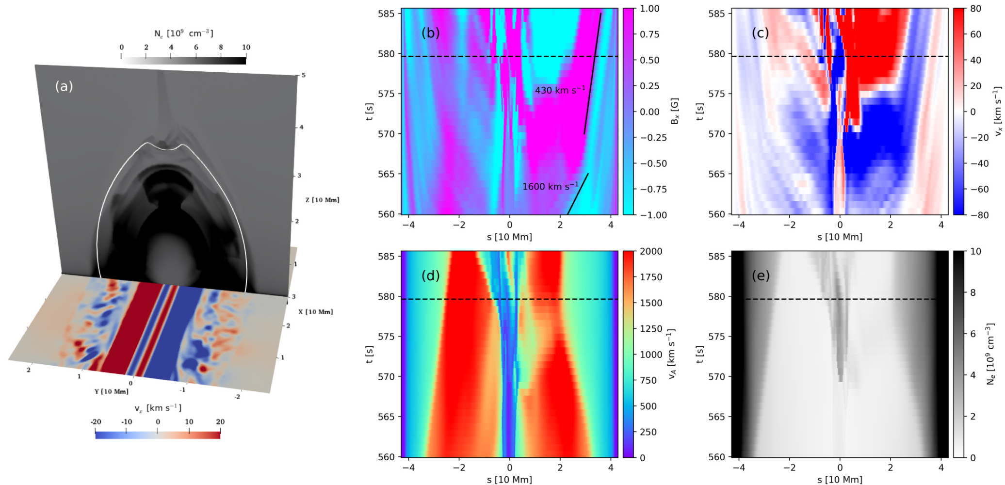
Figure 4. from W. Ruan et al 2023 Astrophys. J. 947 doi:10.3847/1538-4357/ac9b4e https://dx.doi.org/10.3847/1538-4357/ac9b4e © 2023. The Author(s). Published by the American Astronomical Society.
