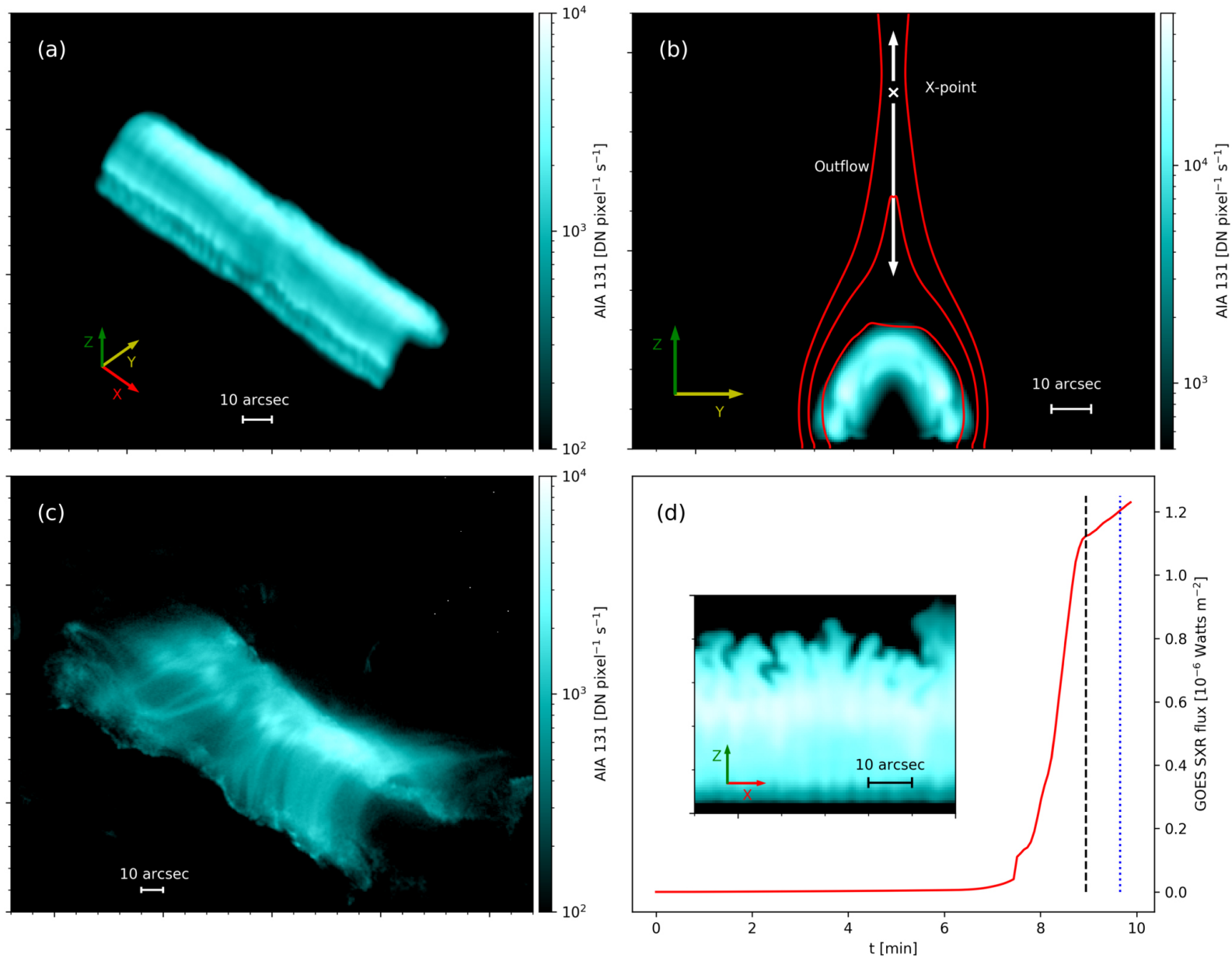
Figure 1. from W. Ruan et al 2023 Astrophys. J. 947 doi:10.3847/1538-4357/ac9b4e https://dx.doi.org/10.3847/1538-4357/ac9b4e © 2023. The Author(s). Published by the American Astronomical Society.
