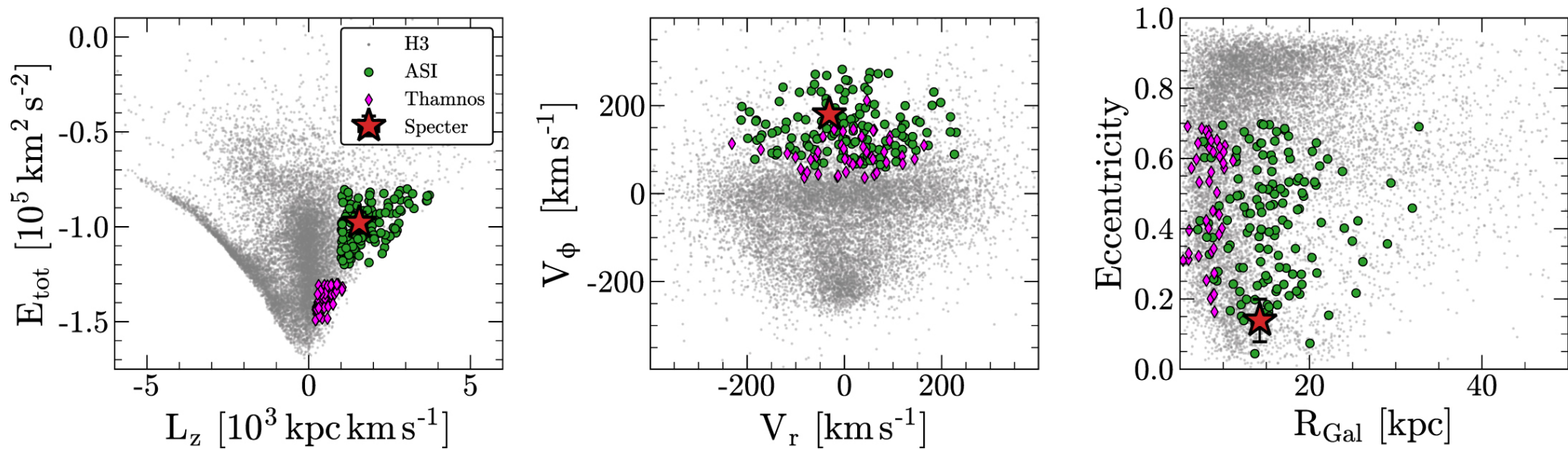
Figure 8. from Vedant Chandra et al 2022 Astrophys. J. 940 doi:10.3847/1538-4357/ac9b4b https://dx.doi.org/10.3847/1538-4357/ac9b4b © 2022. The Author(s). Published by the American Astronomical Society.
