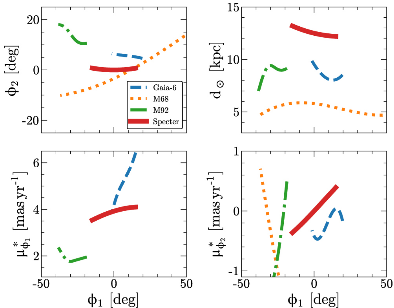
Figure 7. from Vedant Chandra et al 2022 Astrophys. J. 940 doi:10.3847/1538-4357/ac9b4b https://dx.doi.org/10.3847/1538-4357/ac9b4b © 2022. The Author(s). Published by the American Astronomical Society.
