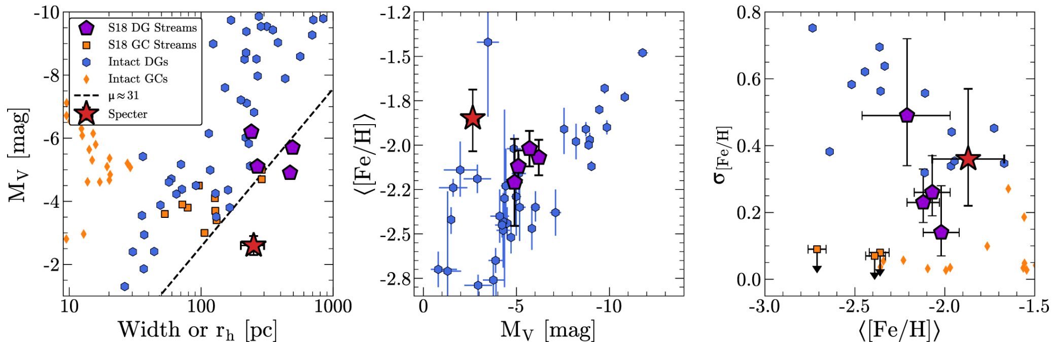
Figure 6. from Vedant Chandra et al 2022 Astrophys. J. 940 doi:10.3847/1538-4357/ac9b4b https://dx.doi.org/10.3847/1538-4357/ac9b4b © 2022. The Author(s). Published by the American Astronomical Society.
