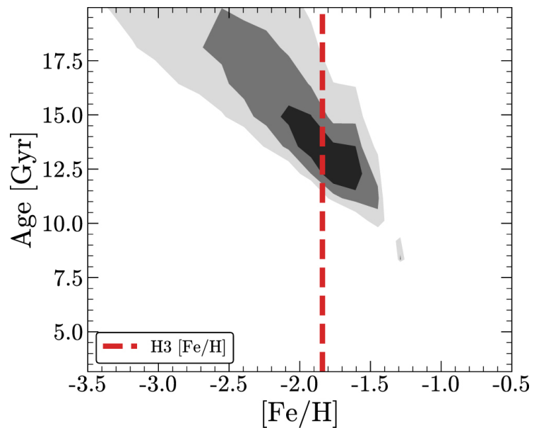
Figure 5. from Vedant Chandra et al 2022 Astrophys. J. 940 doi:10.3847/1538-4357/ac9b4b https://dx.doi.org/10.3847/1538-4357/ac9b4b © 2022. The Author(s). Published by the American Astronomical Society.
