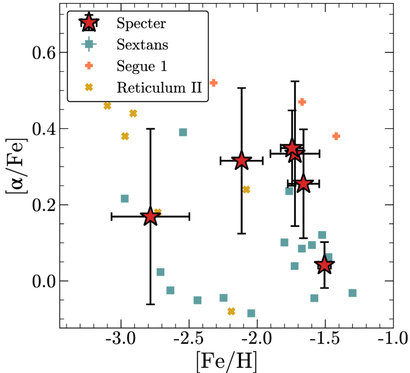
Figure 4. from Vedant Chandra et al 2022 Astrophys. J. 940 doi:10.3847/1538-4357/ac9b4b https://dx.doi.org/10.3847/1538-4357/ac9b4b © 2022. The Author(s). Published by the American Astronomical Society.
