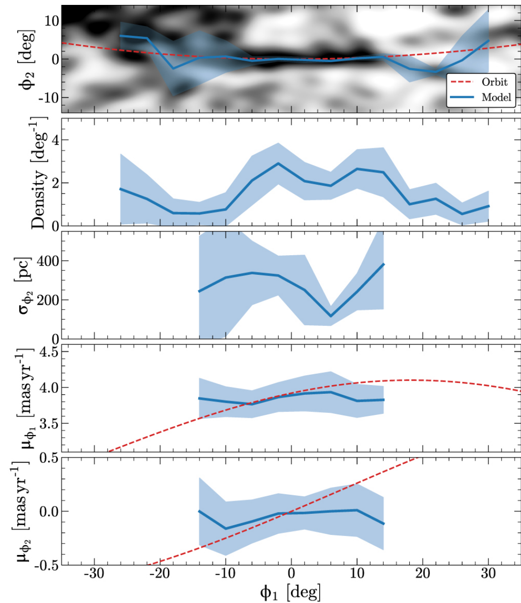
Figure 3. from Vedant Chandra et al 2022 Astrophys. J. 940 doi:10.3847/1538-4357/ac9b4b https://dx.doi.org/10.3847/1538-4357/ac9b4b © 2022. The Author(s). Published by the American Astronomical Society.
