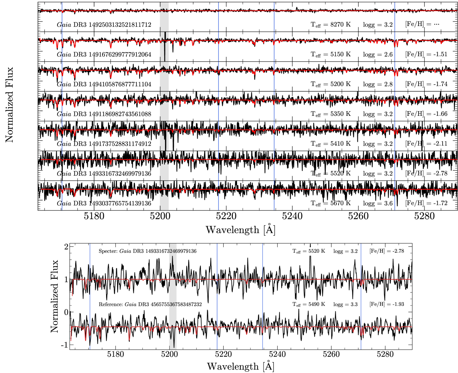
Figure 10. from Vedant Chandra et al 2022 Astrophys. J. 940 doi:10.3847/1538-4357/ac9b4b https://dx.doi.org/10.3847/1538-4357/ac9b4b © 2022. The Author(s). Published by the American Astronomical Society.
