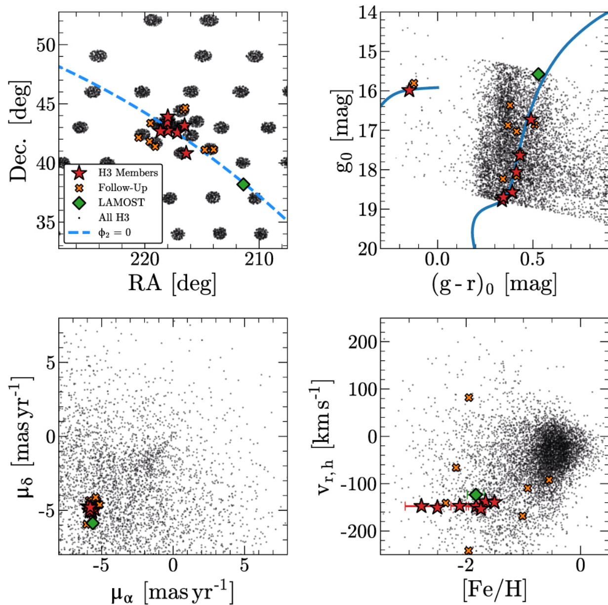
Figure 1. from Vedant Chandra et al 2022 Astrophys. J. 940 doi:10.3847/1538-4357/ac9b4b https://dx.doi.org/10.3847/1538-4357/ac9b4b © 2022. The Author(s). Published by the American Astronomical Society.
