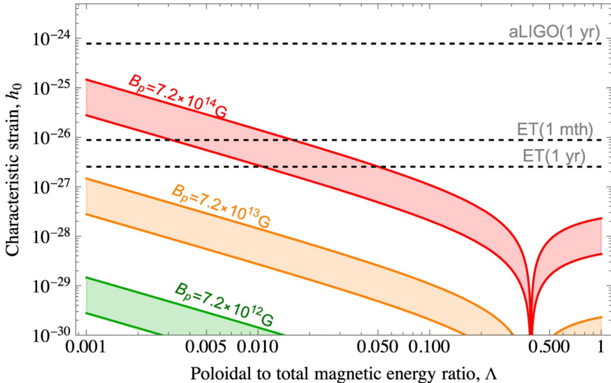
Figure 5. from Arthur G. Suvorov and Kostas Glampedakis 2022 Astrophys. J. 940 doi:10.3847/1538-4357/ac9b48 https://dx.doi.org/10.3847/1538-4357/ac9b48 © 2022. The Author(s). Published by the American Astronomical Society.
