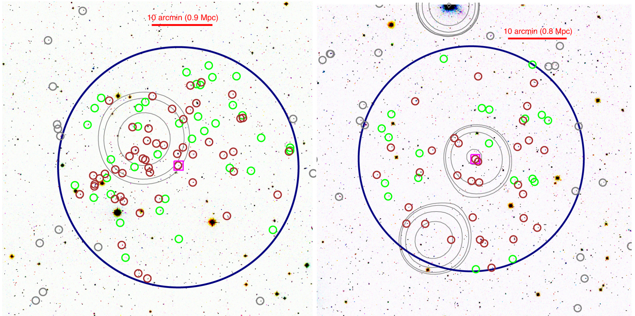
Figure 3. from Kaiyuan Chen et al 2022 Astrophys. J. 940 doi:10.3847/1538-4357/ac9b44 https://dx.doi.org/10.3847/1538-4357/ac9b44 © 2022. The Author(s). Published by the American Astronomical Society.
