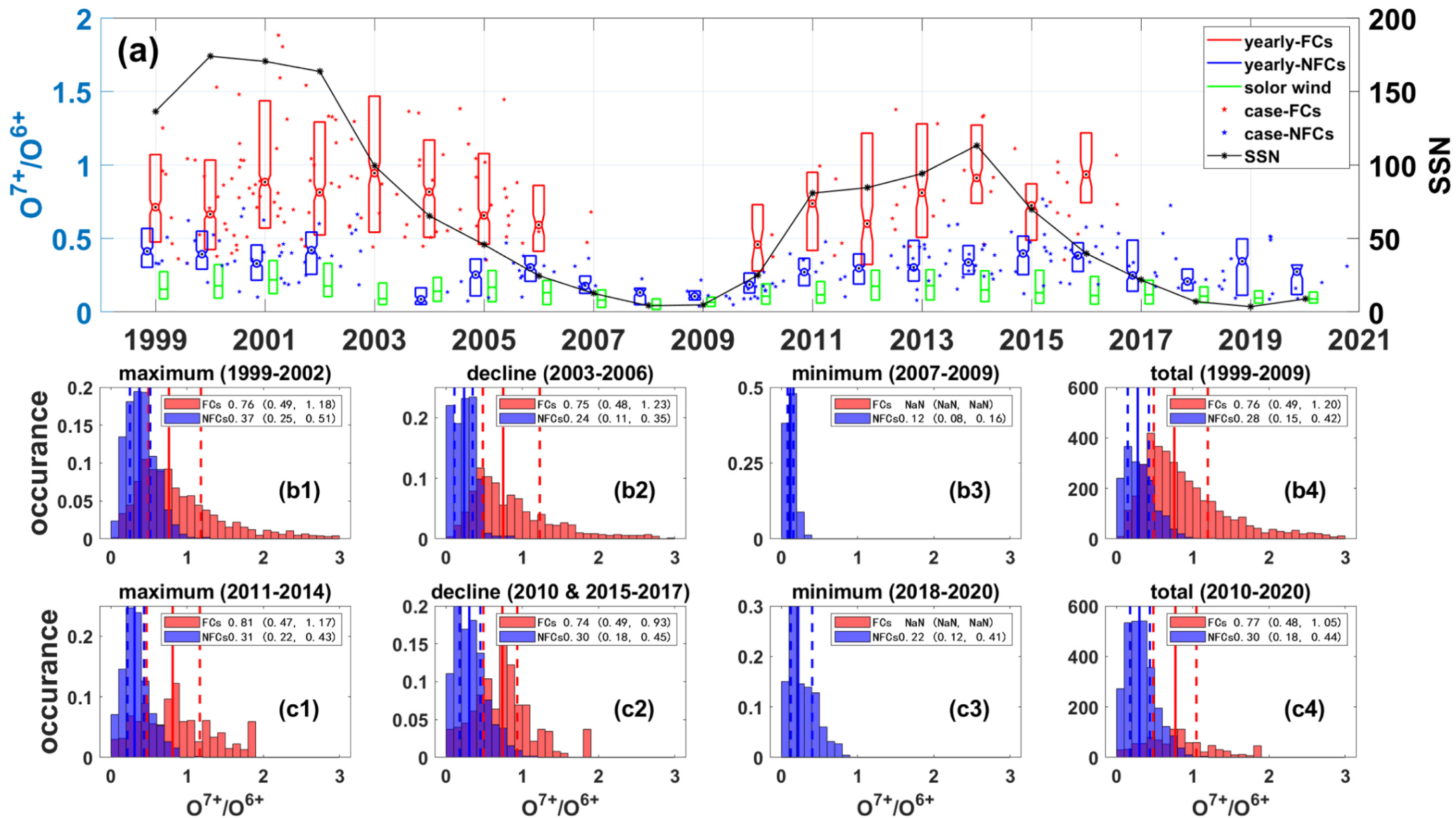
Figure 4. from Xinzheng Shi et al 2022 Astrophys. J. 940 doi:10.3847/1538-4357/ac9b20 https://dx.doi.org/10.3847/1538-4357/ac9b20 © 2022. The Author(s). Published by the American Astronomical Society.
