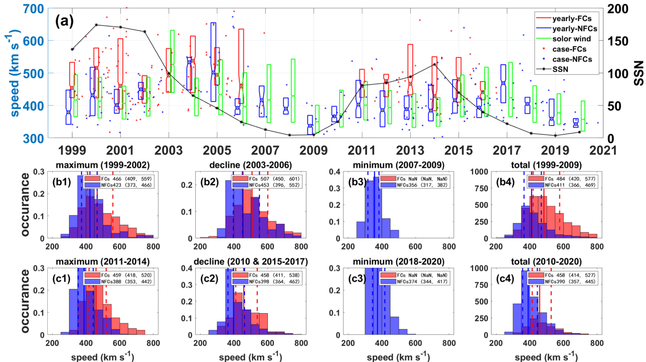
Figure 2. from Xinzheng Shi et al 2022 Astrophys. J. 940 doi:10.3847/1538-4357/ac9b20 https://dx.doi.org/10.3847/1538-4357/ac9b20 © 2022. The Author(s). Published by the American Astronomical Society.
