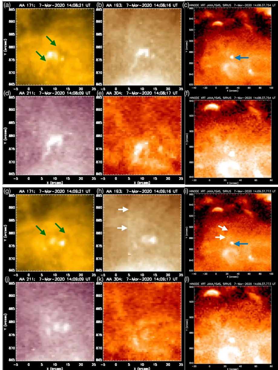
Figure 3. from Alphonse C. Sterling et al 2022 Astrophys. J. 940 doi:10.3847/1538-4357/ac9960 https://dx.doi.org/10.3847/1538-4357/ac9960 © 2022. The Author(s). Published by the American Astronomical Society.
