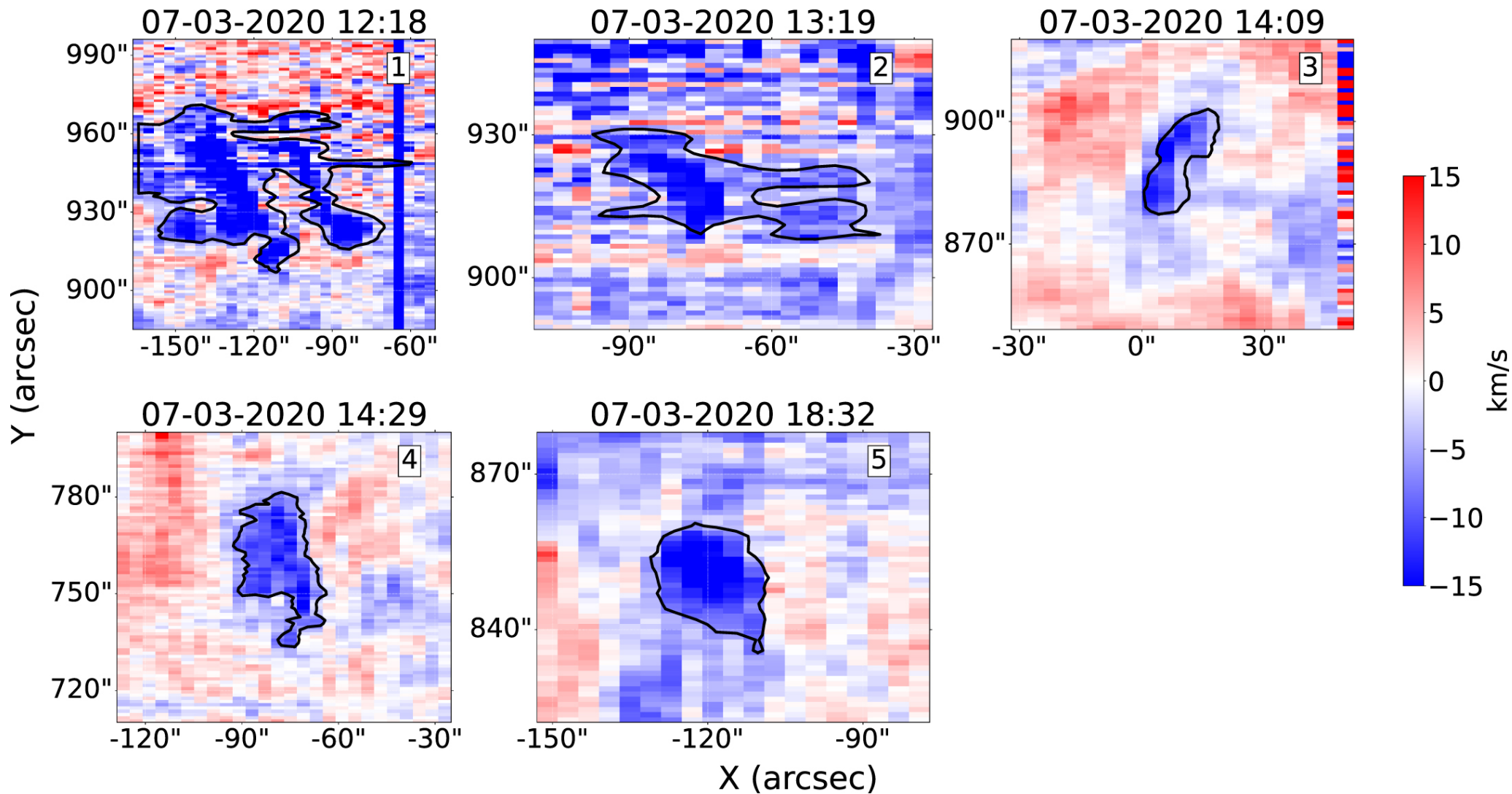
Figure 1. from Alphonse C. Sterling et al 2022 Astrophys. J. 940 doi:10.3847/1538-4357/ac9960 https://dx.doi.org/10.3847/1538-4357/ac9960 © 2022. The Author(s). Published by the American Astronomical Society.
