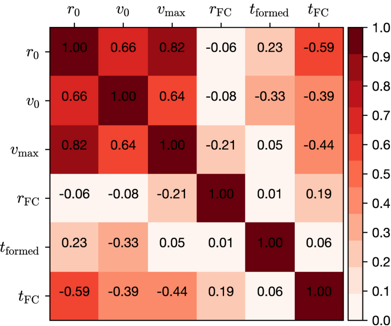
Figure 5. from Hannah Jhee et al 2022 Astrophys. J. 940 doi:10.3847/1538-4357/ac990a https://dx.doi.org/10.3847/1538-4357/ac990a © 2022. The Author(s). Published by the American Astronomical Society.
