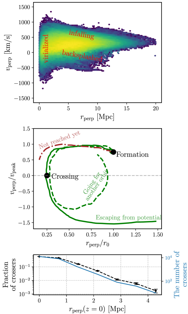
Figure 3. from Hannah Jhee et al 2022 Astrophys. J. 940 doi:10.3847/1538-4357/ac990a https://dx.doi.org/10.3847/1538-4357/ac990a © 2022. The Author(s). Published by the American Astronomical Society.
