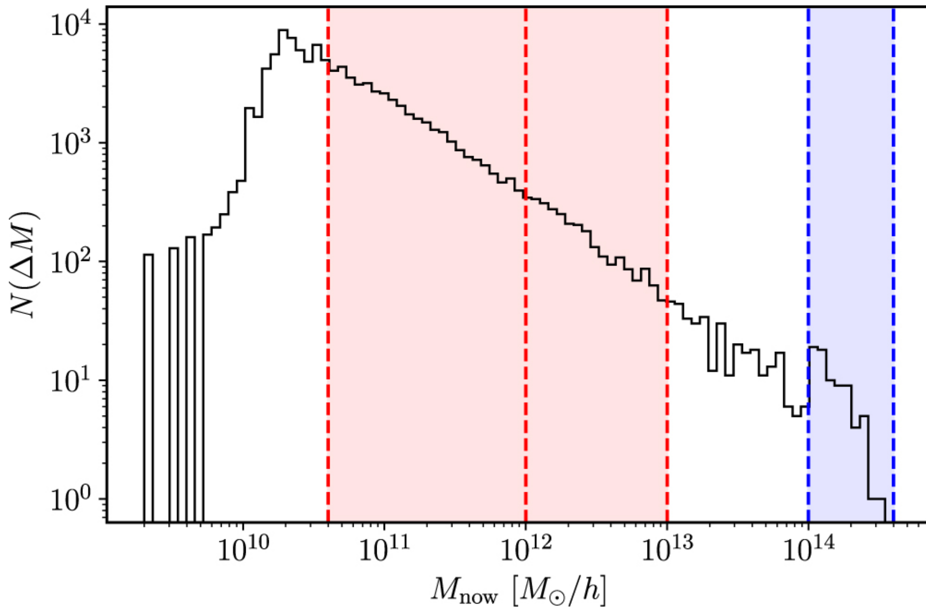
Figure 2. from Hannah Jhee et al 2022 Astrophys. J. 940 doi:10.3847/1538-4357/ac990a https://dx.doi.org/10.3847/1538-4357/ac990a © 2022. The Author(s). Published by the American Astronomical Society.
