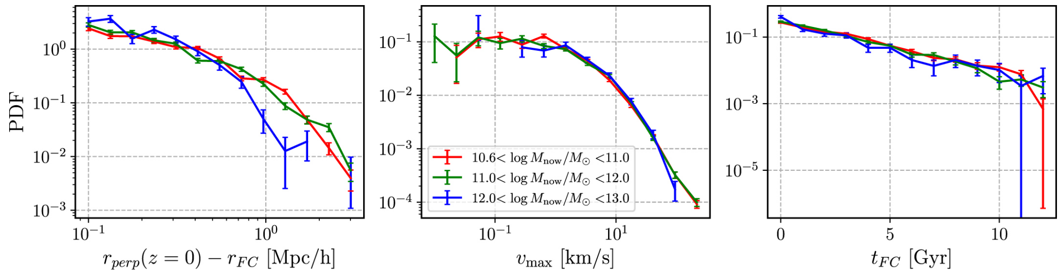
Figure 15. from Hannah Jhee et al 2022 Astrophys. J. 940 doi:10.3847/1538-4357/ac990a https://dx.doi.org/10.3847/1538-4357/ac990a © 2022. The Author(s). Published by the American Astronomical Society.
