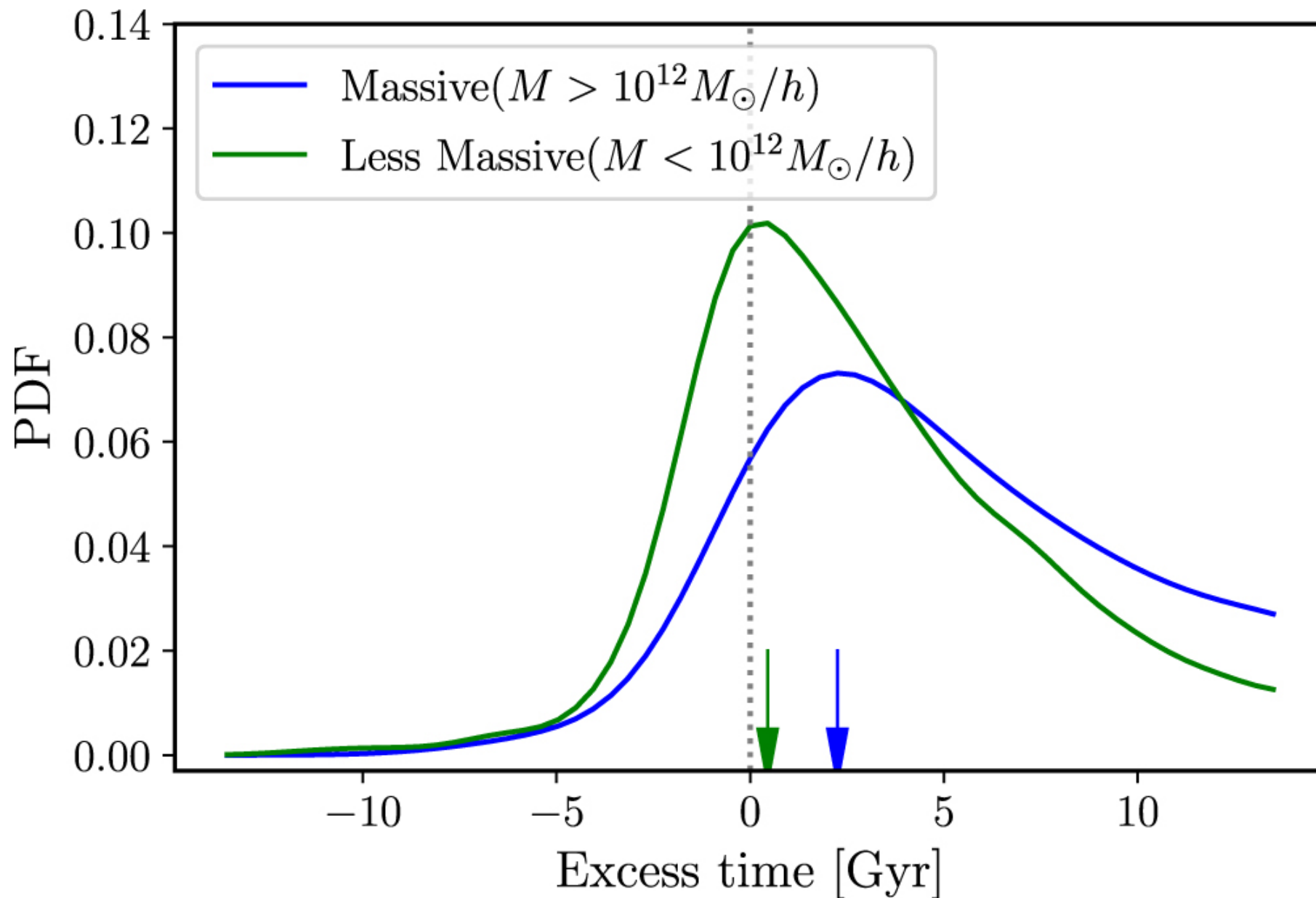
Figure 13. from Hannah Jhee et al 2022 Astrophys. J. 940 doi:10.3847/1538-4357/ac990a https://dx.doi.org/10.3847/1538-4357/ac990a © 2022. The Author(s). Published by the American Astronomical Society.
