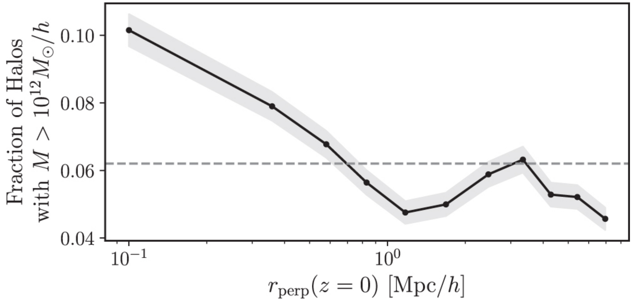
Figure 12. from Hannah Jhee et al 2022 Astrophys. J. 940 doi:10.3847/1538-4357/ac990a https://dx.doi.org/10.3847/1538-4357/ac990a © 2022. The Author(s). Published by the American Astronomical Society.
