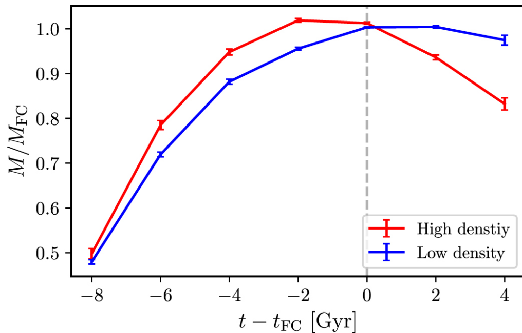
Figure 11. from Hannah Jhee et al 2022 Astrophys. J. 940 doi:10.3847/1538-4357/ac990a https://dx.doi.org/10.3847/1538-4357/ac990a © 2022. The Author(s). Published by the American Astronomical Society.
