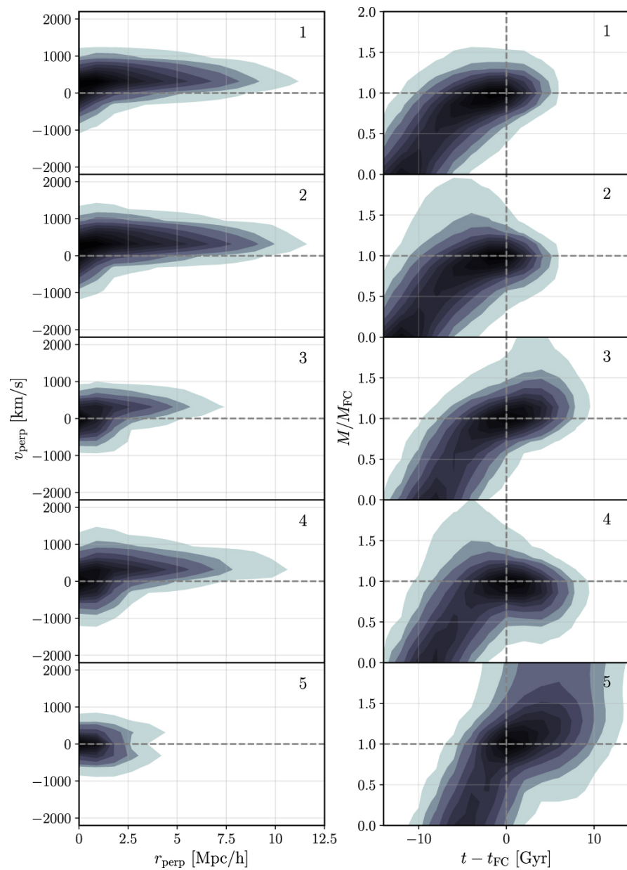
Figure 10. from Hannah Jhee et al 2022 Astrophys. J. 940 doi:10.3847/1538-4357/ac990a https://dx.doi.org/10.3847/1538-4357/ac990a © 2022. The Author(s). Published by the American Astronomical Society.
