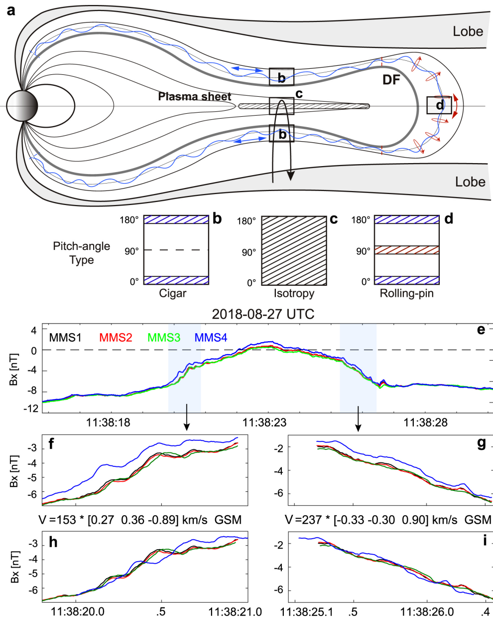
Figure 3. from R. J. He et al 2022 Astrophys. J. 940 doi:10.3847/1538-4357/ac9669 https://dx.doi.org/10.3847/1538-4357/ac9669 © 2022. The Author(s). Published by the American Astronomical Society.
