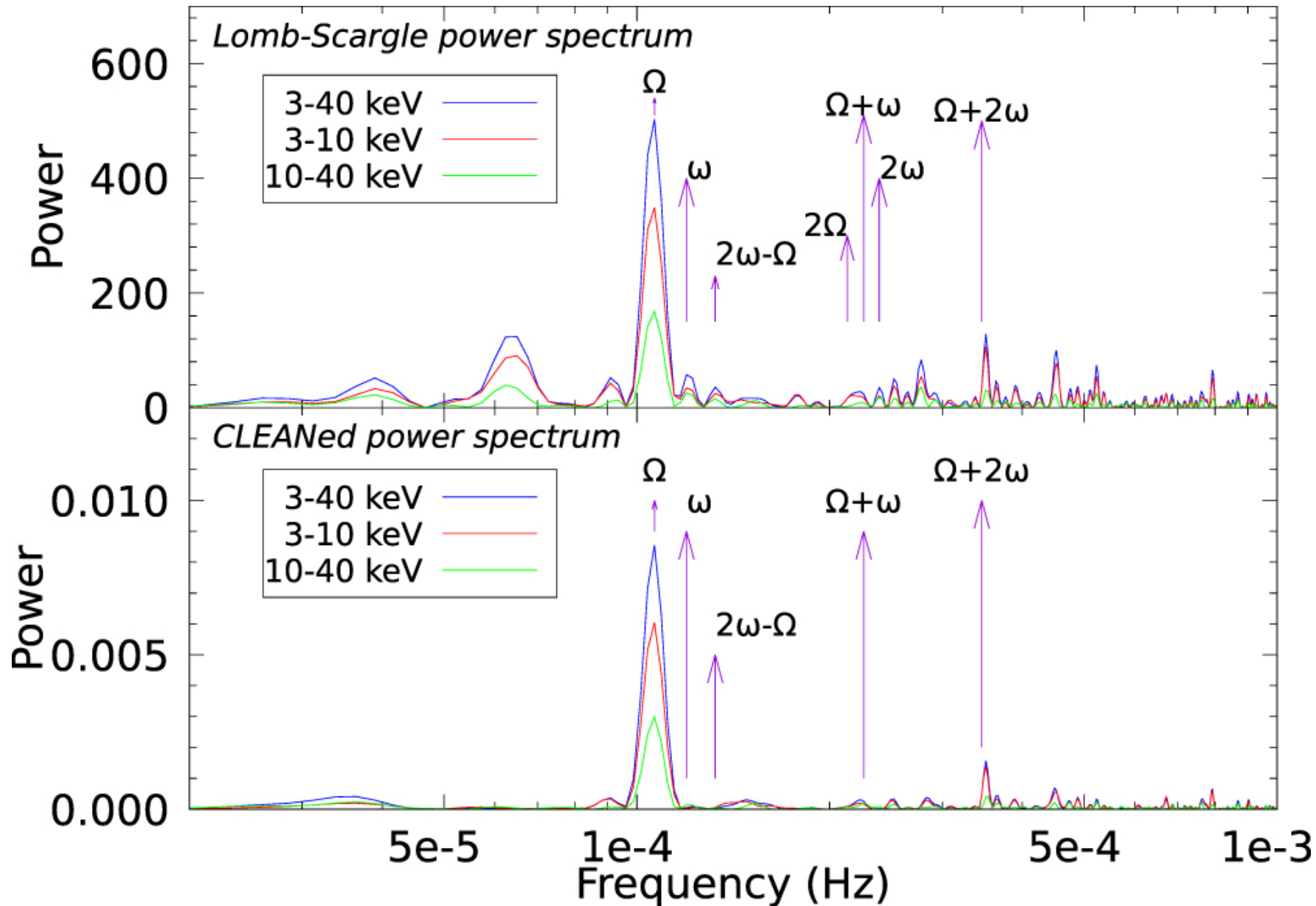
Figure 2. from Anirban Dutta and Vikram Rana 2022 Astrophys. J. 940 doi:10.3847/1538-4357/ac9587 https://dx.doi.org/10.3847/1538-4357/ac9587 © 2022. The Author(s). Published by the American Astronomical Society.
